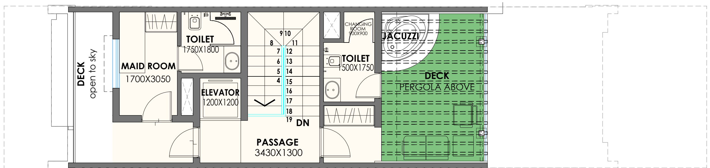
THIRD FLOOR PLAN
